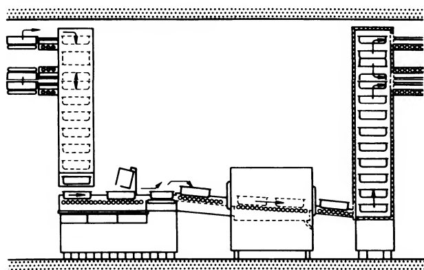
5 Container movement in the Contiport system
